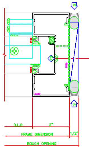
403 JAMB 403 SHEARBLOCK
