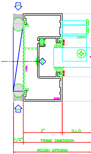
402 JAMB 403 SHEARBLOCK
